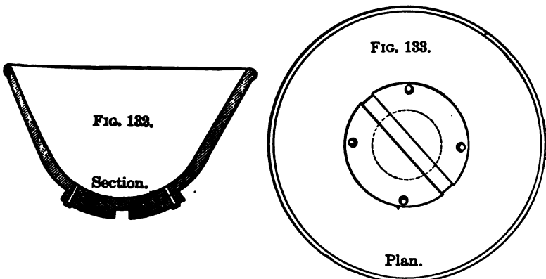
SECTION/L SLAG-POT.
